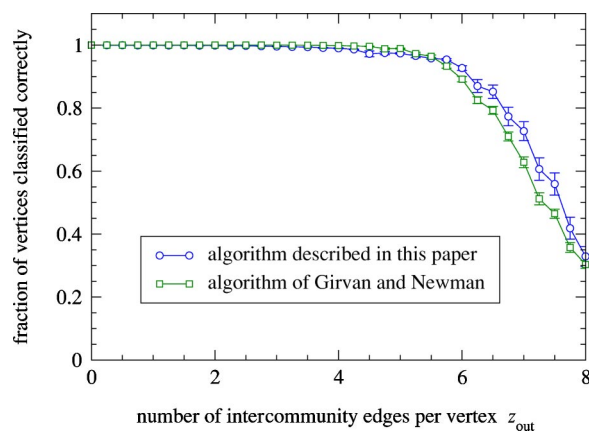
FIG. 1. The fraction of vertices correctly identified by our algorithms in the computer-generated graphs described in the text. The two curves show results for our algorithm (circles) and for the algorithm of Girvan and Newman [5] (squares). Each point is an average over 100 graphs.
